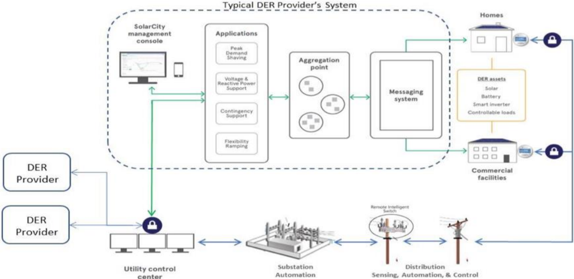
Figure 27 DER Aggregator & Utility Communications/Security Interfaces
